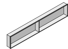
CONTAINER + LED 1850 x 80 x H 300 mm 72"83 x 3"15 x H 11"81
